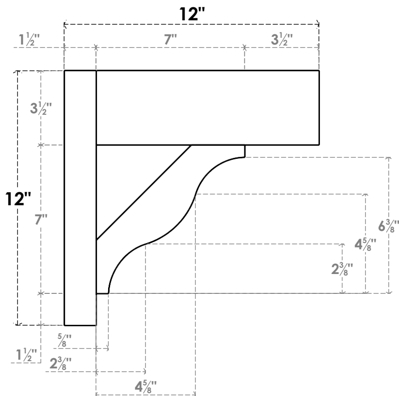
SIDE PROFILE
